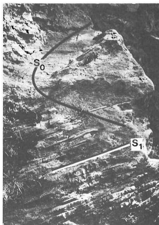
Fig. 17. F1 fold in the Jordalen locality where bedding is folded, and S1 is defined by flattened quartzite pebbles in the Jordalen Member (999037). Looking south.
