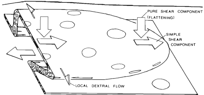
Fig. 21. Schematic illustration of a sheath-fold formed during thrusting to the east. Flattening strain during the development of the fold causes local lateral flow, either dextral or sinistral.
