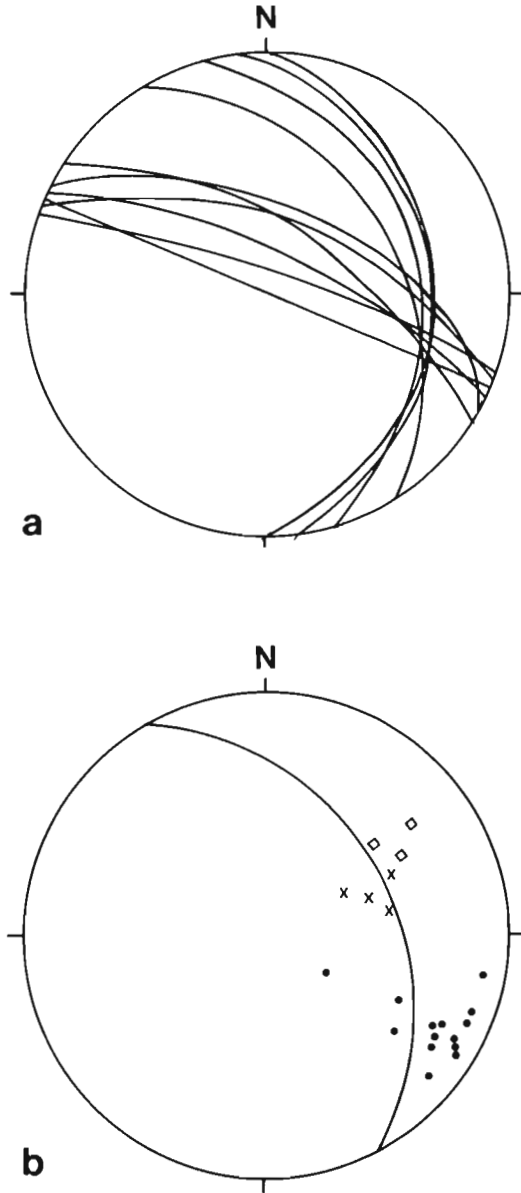
Fig. 19. (a) Measurements of bedding around the lower hinge zone of the F1 fold at the Sandvikshytten locality indicates a theoretical fold axis plunging to the E or ESE. (b) Orientation of mesoscopic fold axes in the Sandvikshytten locality (dots), Jordalen locality (crosses) and north of Ulriken (squares). The great circle indicates the average plane of foliation in the area (330/35NE).
