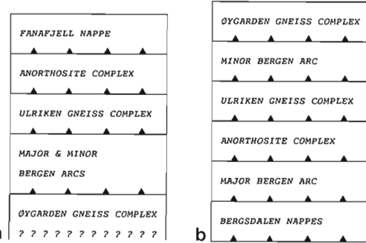
Fig. 2. Two different interpretations of the nappe stratigraphy of the Bergen Arcs; (a) from Sturt & Thon (1978); (b) interpretation based on large-scale asymmetrical folding of the Bergen Arcs (see text and Fig. 22). Note that the Fanafjell Nappe in Fig. 2a is part of the Major Bergen Arc in Fig. 2b.
